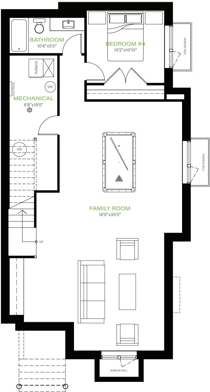
Basement Development
